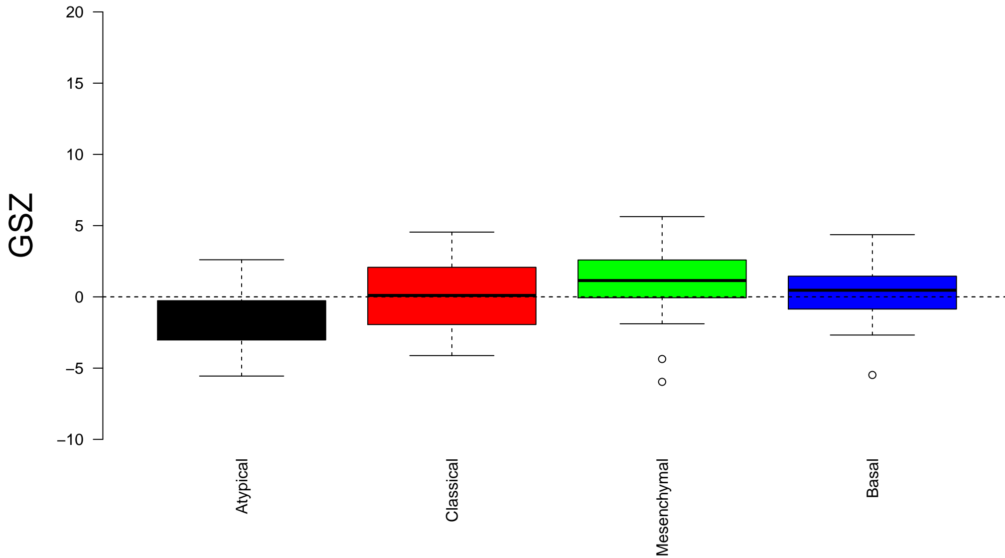
Christensen_hypermethylated_in_grade3_astrocytoma
